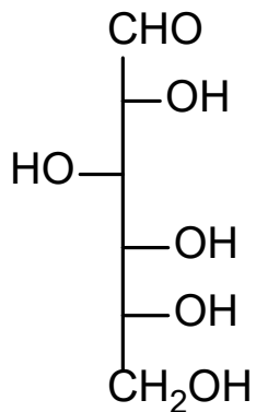
D-glucose
